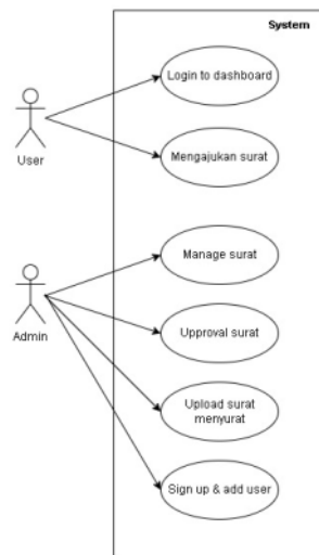
Gambar 2. Usecase Diagram
