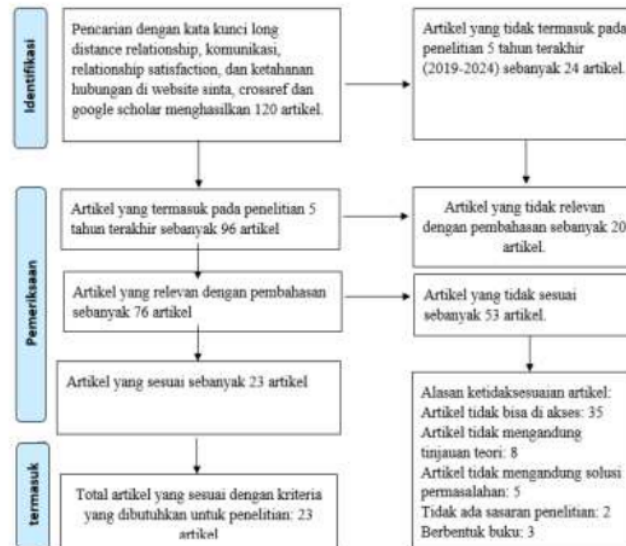
Gambar 1: Langkah-Langkah SLR
