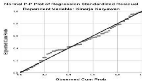
Gambar 1 Grafik Normal P-P Plot
