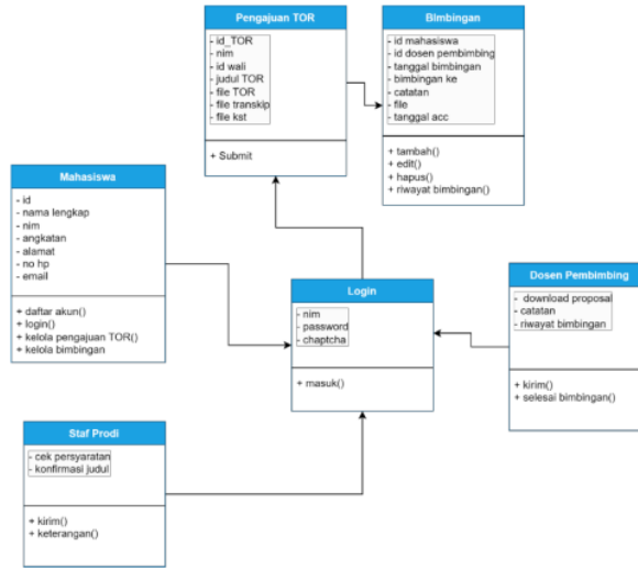
Gambar 3.4 Class Diagram
