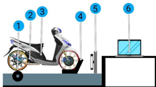
Gambar 3.1 Setting Peralatan Penelitian
